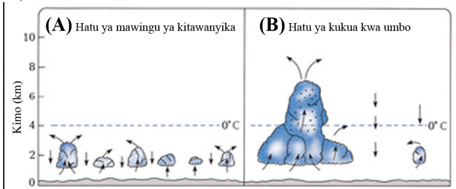
Umbo 19: (A) vipande vidogo vidogo vya mawingu vilivyojitenga (cumulus clouds). (B) Wakati mawingu madogo madogo yanapoungana pamoja, yanajirundika na wingu kubwa linaongezeka, kwahiyo wingu limesharundikana. Matone ya mvua yanayodondoka yanaonyeshwa kwa alama ya • (The Atmosphere, Anthes and others, ukurasa wa, 269.)
